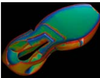
Scanned geometry with false color curvature mapping.
