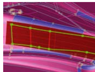
A shared base surface is assigned to the three labeled faces
